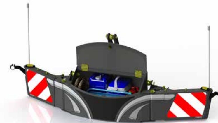
Bumper with integrated storage box
